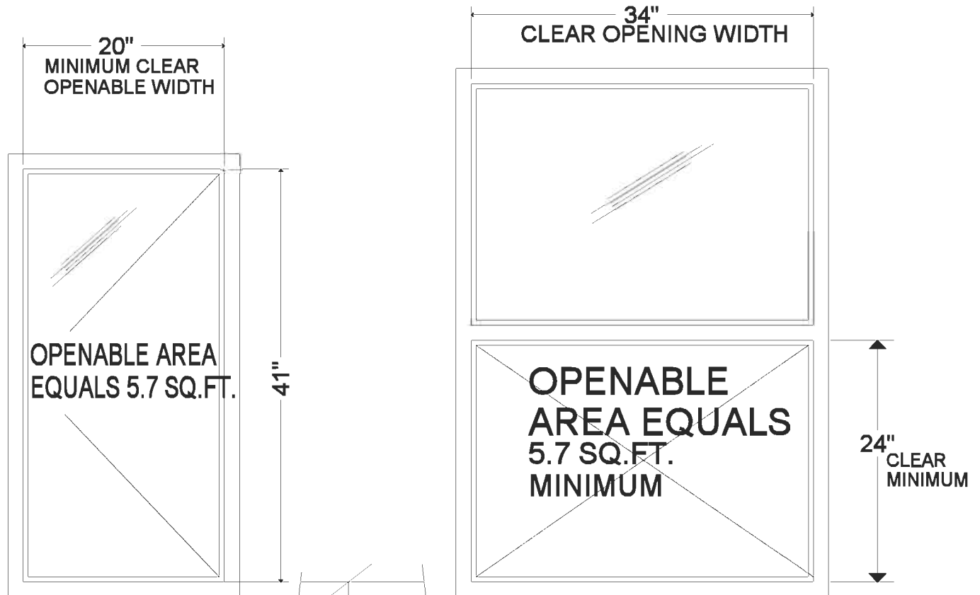
MINIMUM SIZE WINDOW FOR A 20 INCH CLEAR WIDTH
