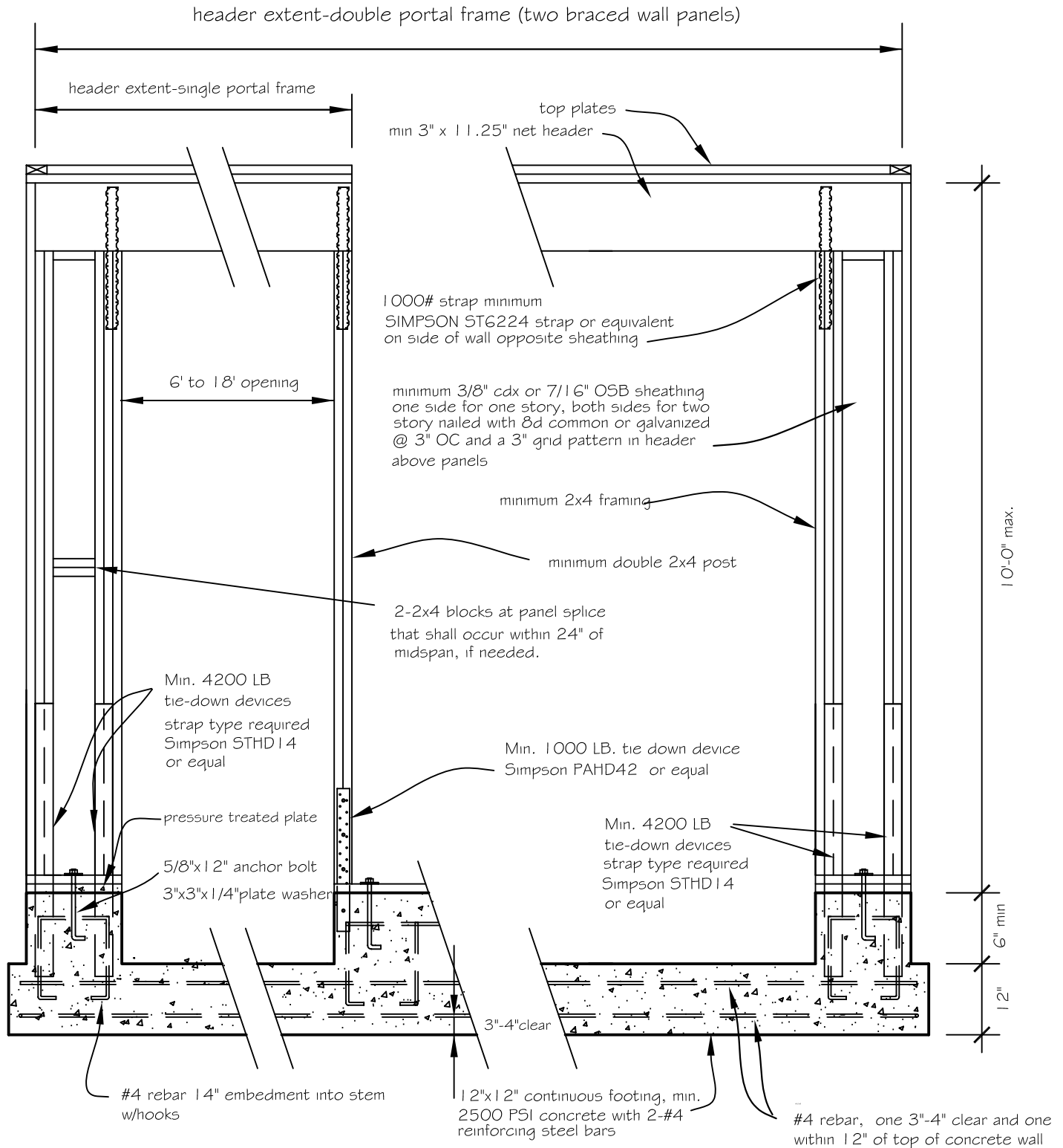
Portal Frame with hold-downs
