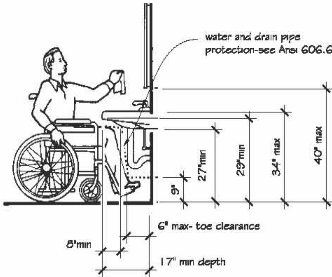
Figure 1 Lavatory Clearances
