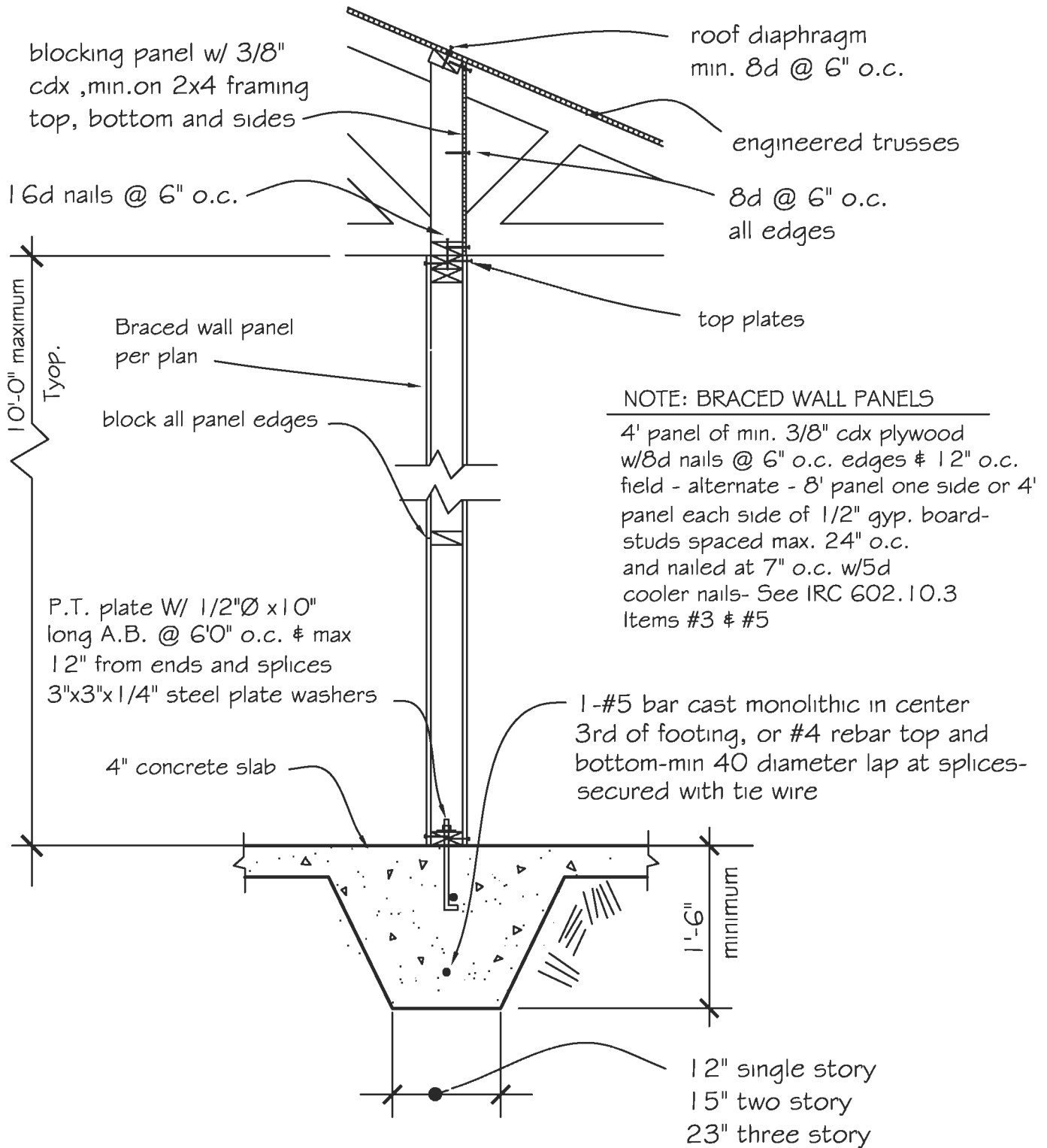
Interior Braced Wall Panels w/footing (w/joists or rafters perpendicular to panels)
