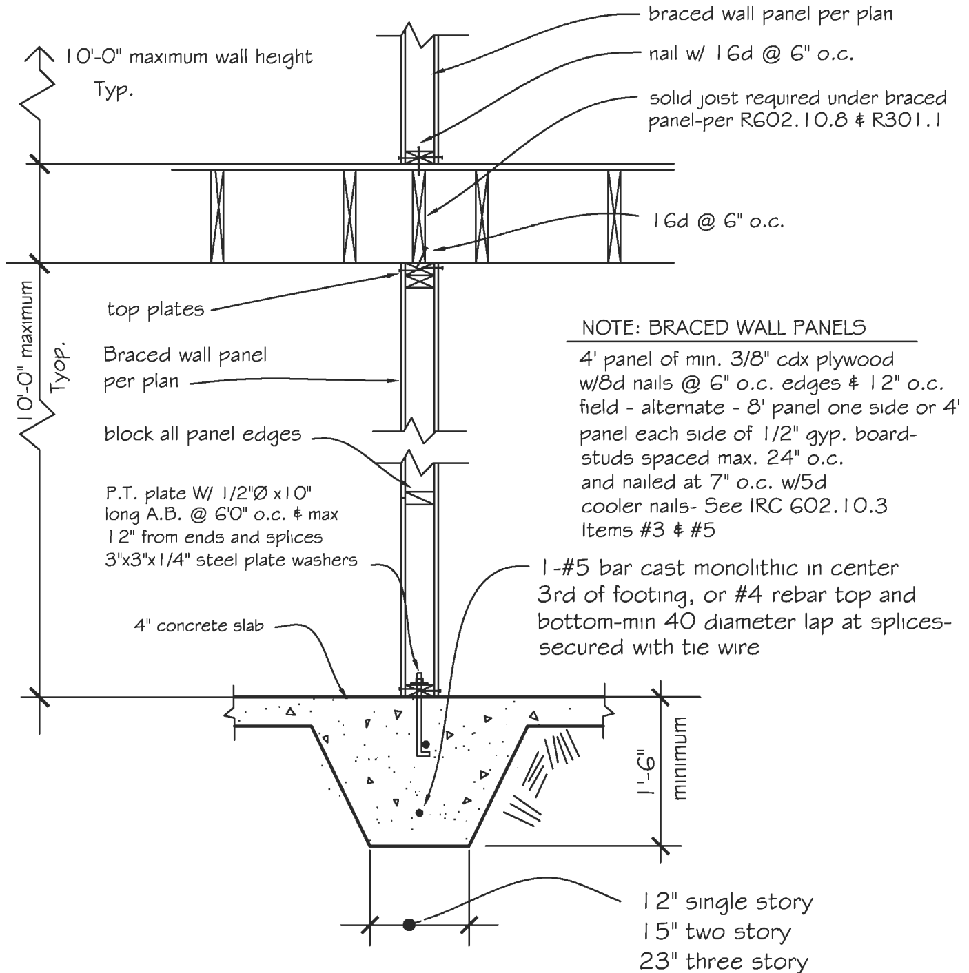
Interior Braced Wall Panels w/footing (w/floor above)
