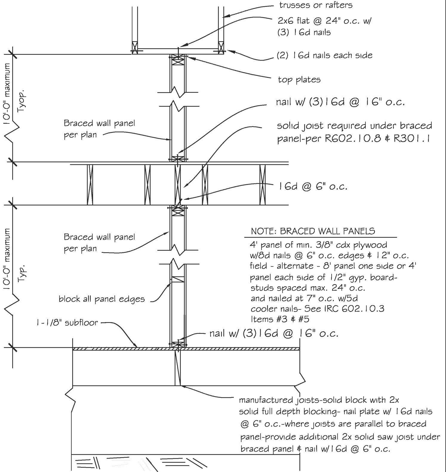
Interior Braced Wall Panels (w/trusses or rafters parallel to panels)
