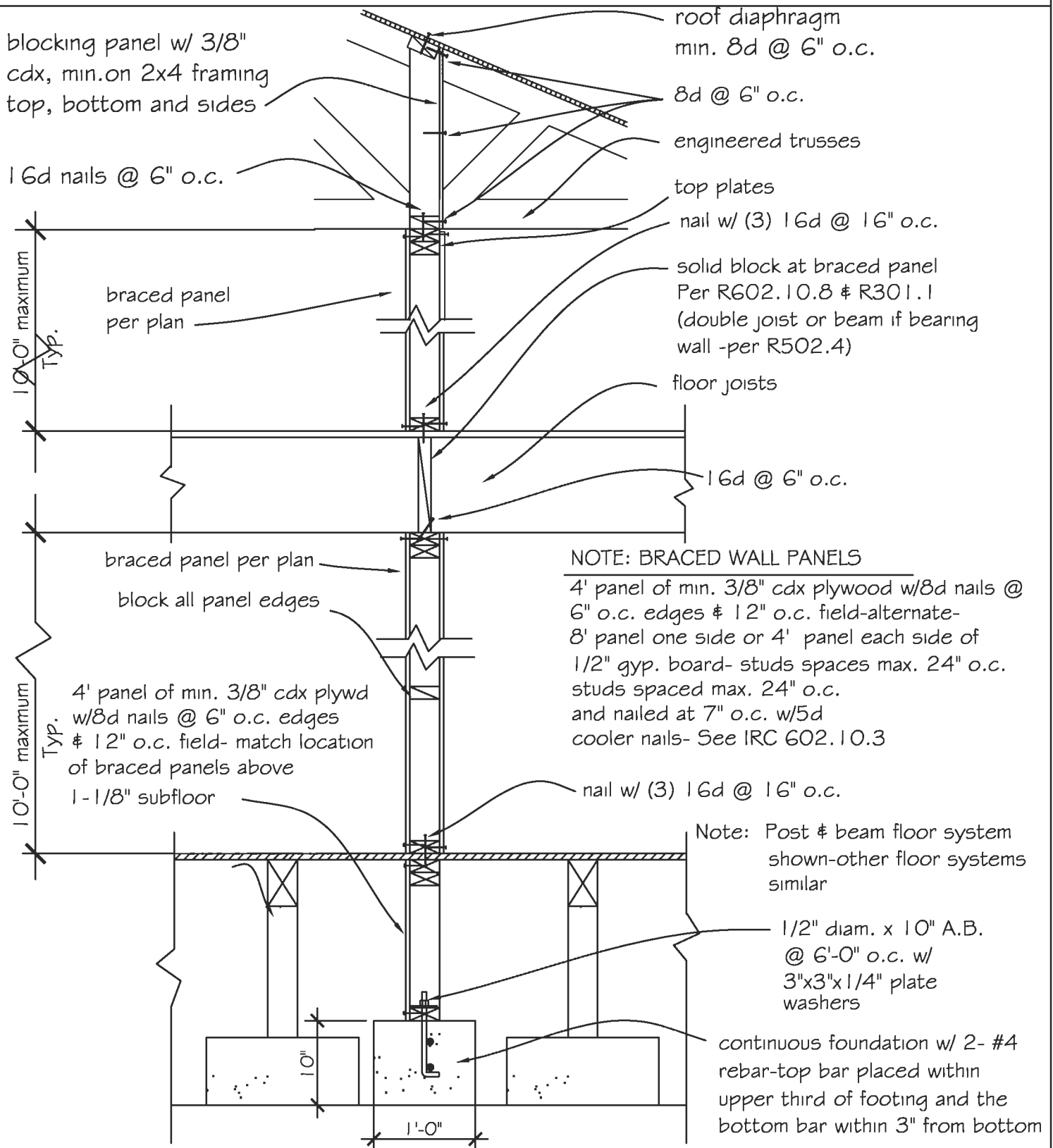
Interior Braced Wall Panels (w/trusses or rafters perpendicular to panels)
