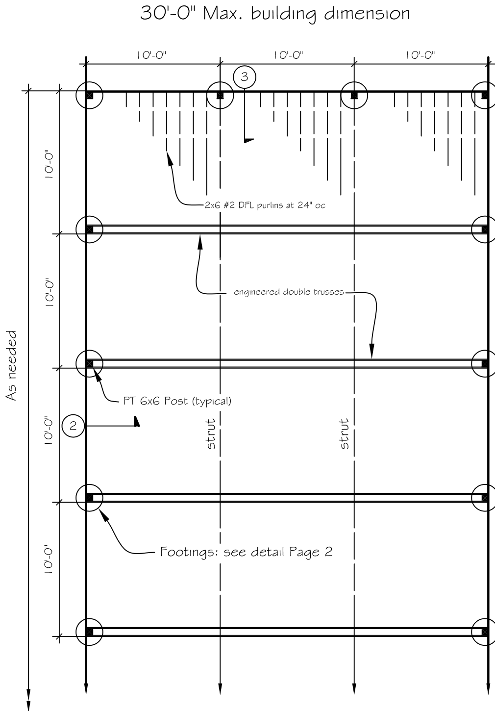
Floor Plan for 10' sidewall
