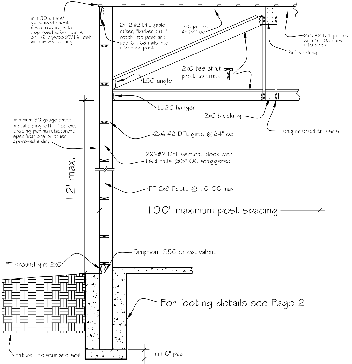
12'0" SIDEWALL (MAX) GABLE END DETAIL
