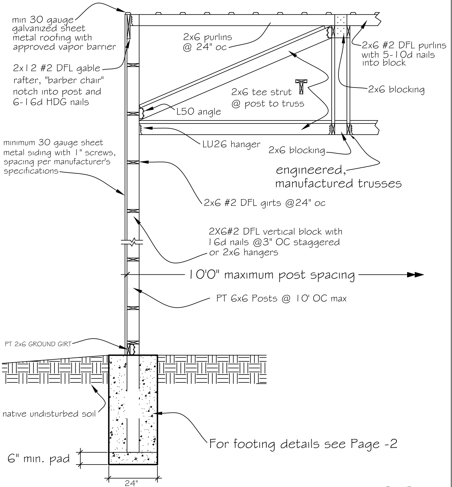
10'0" SIDEWALL (MAX) GABLE END DETAIL
