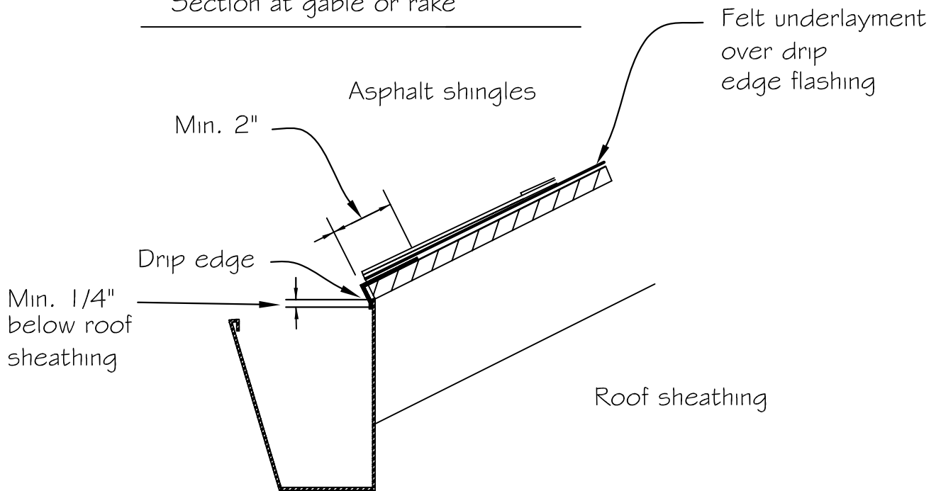
Section at gable or rake
