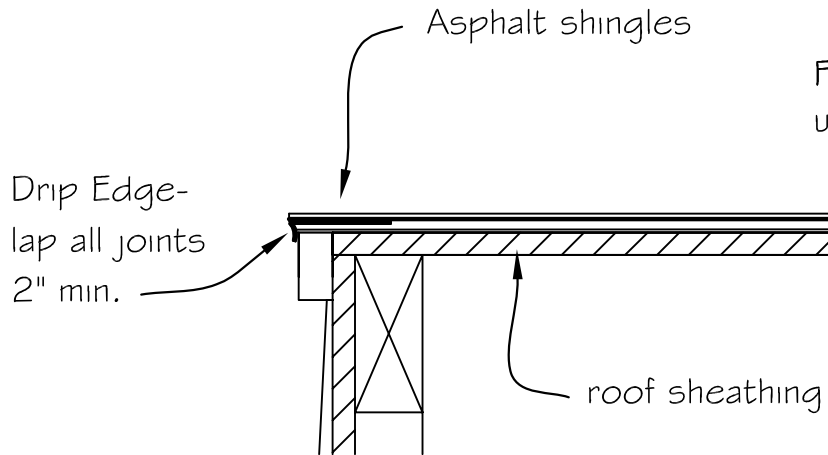
Section at gable or rake
